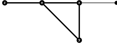
FIGURE 2. A thin graph whereby \langle N[v] \rangle is not thin. The S -classes in \langle N[v] \rangle are S_v(v) = \{v\} , S_v(z) = \{z\} and S_v(x) = S_v(y) = \{x, y\} .
