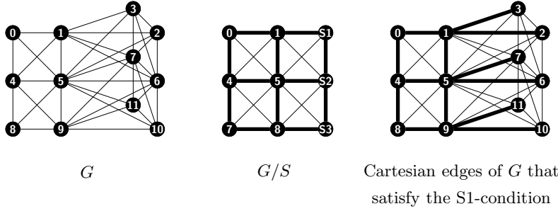
FIGURE 3. This figure shows how we identify (a couple of) Cartesian edges that satisfy the S1-condition . Given a graph G compute its quotient graph G/S , decompose G/S w.r.t. to its strong prime factors. Since G/S is thin the Cartesian edges in G/S are uniquely determined. Apply now Lemma 2.9 to identify all Cartesian edges in G that satisfy the S1-condition in G/S .
