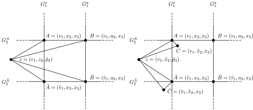
FIGURE 12. Left: Case 2.A.i. and ii.. Right: Case 2.B.i. and ii.
