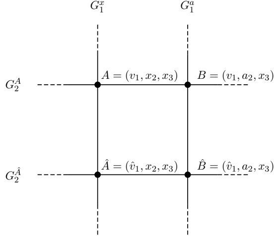
FIGURE 10. General notation of the chosen square A\hat{A}\hat{B}B .
