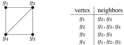
Figure 4: Adjacency list representation of G
