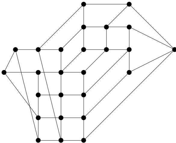
Figure 2: A semi-median graph
