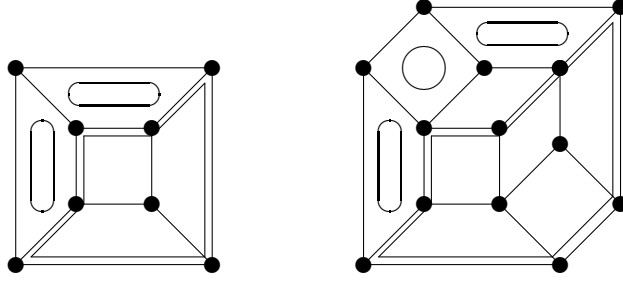
Figure 3: A connected expansion
