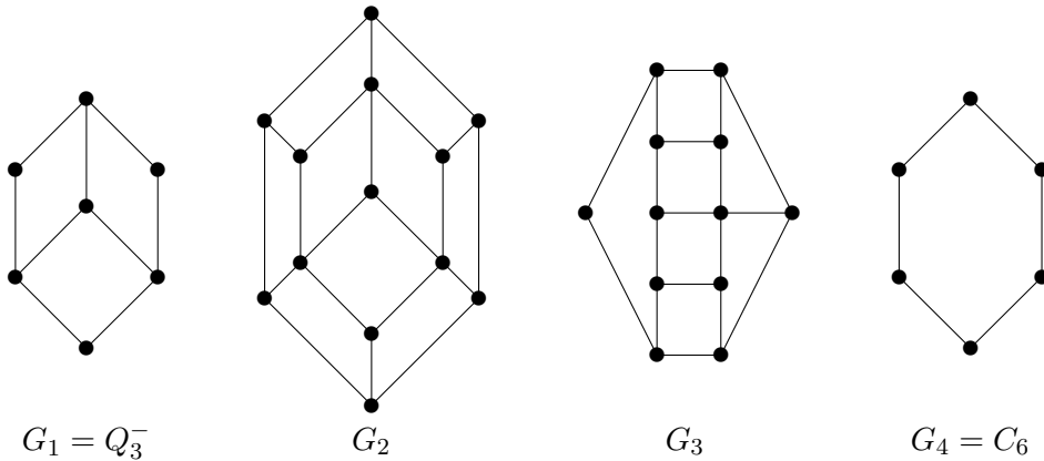
Figure 1: Partial cubes
