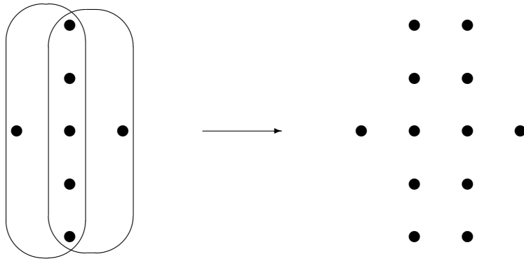
Figure 1: Connected expansion yielding a non semi-median graph
