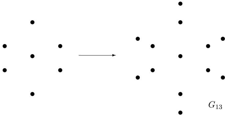
Figure 2: An isometric expansion of Q_3^-
