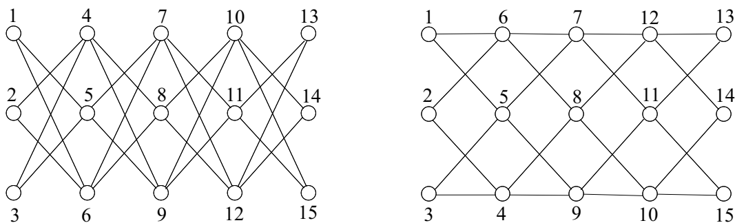
Figure 3: Isomorphic direct products.
